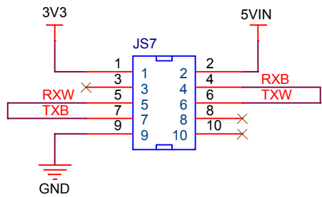
UART Connector
